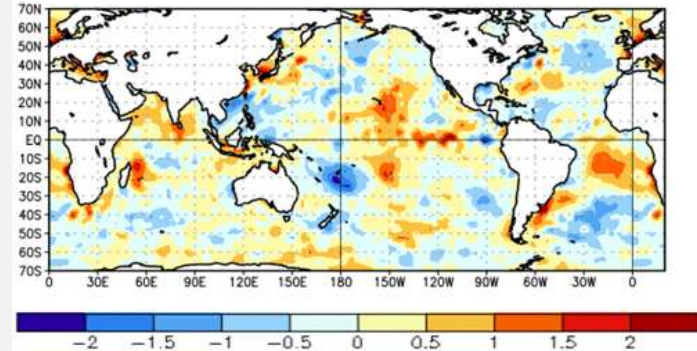
The latest weekly SST departures are:
