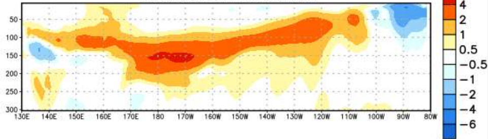
EQ. Subsurface Temperature Anomalies (deg C) Pentad centered on 18 APR 2018
