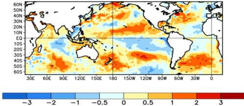
Average SST Anomalies 25 MAR 2018 – 21 APR 2018
